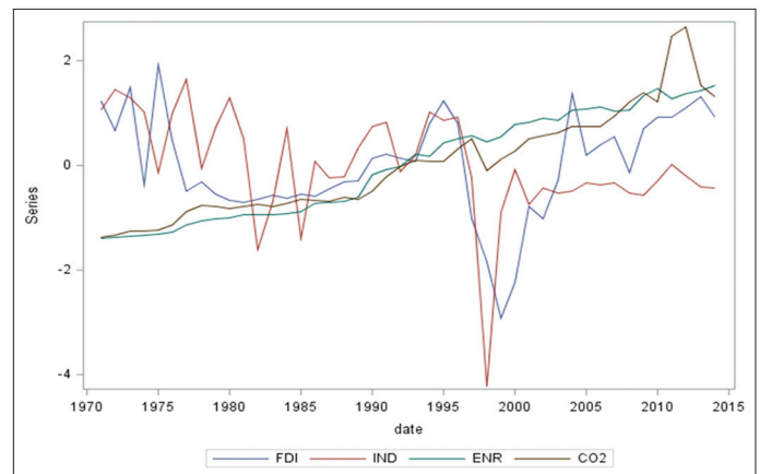
Figure 4: Plot of data foreign direct investment, industry growth, energy use, and carbon dioxide emissions after standardization
